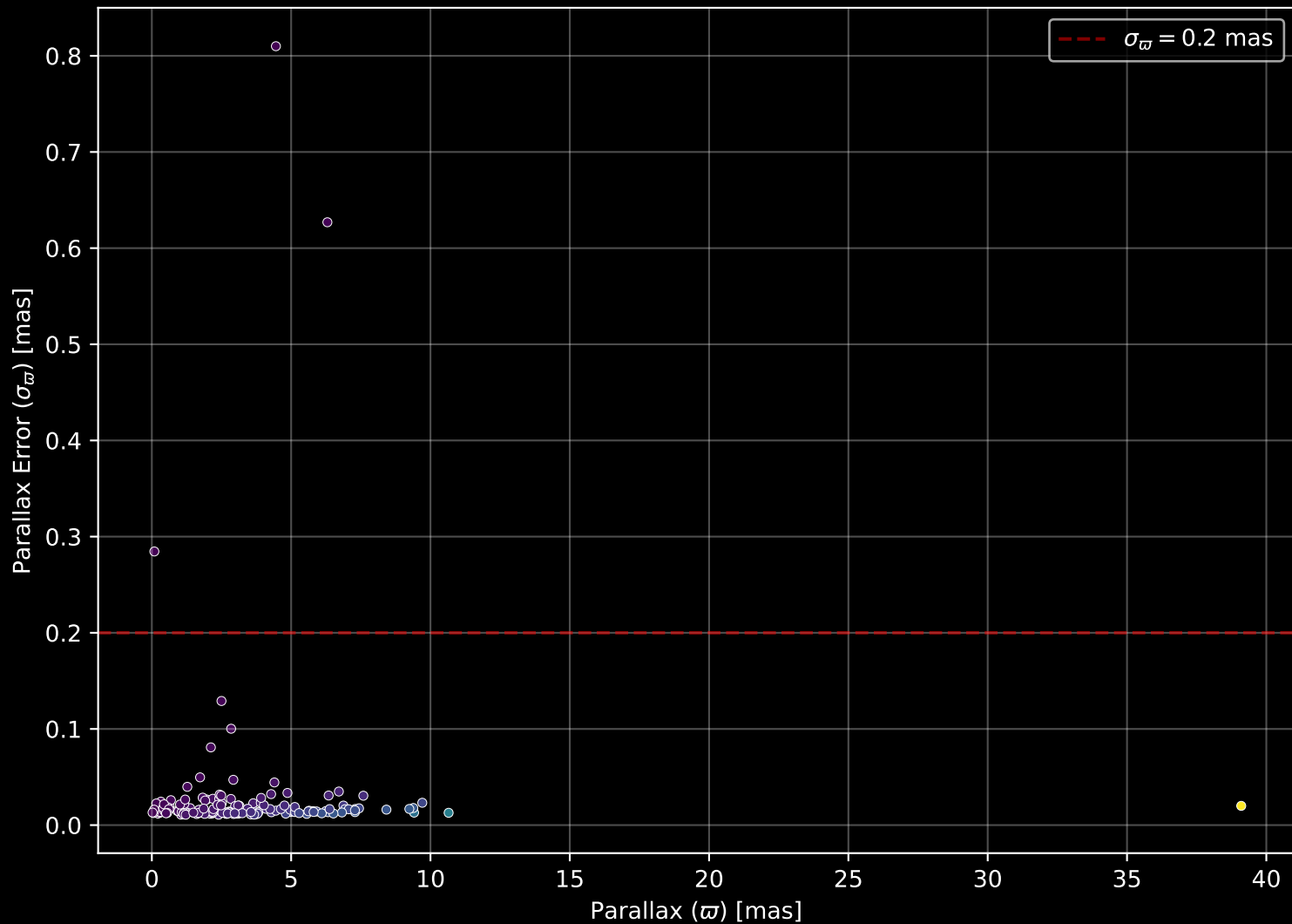
APOGEE DR17 Field: [038+48_MGA] Parallax Quality (n= 159)
