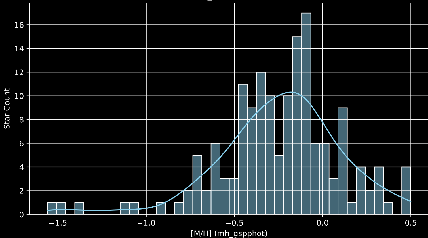
APOGEE DR17 Field: [038+48_MGA [M/H] (mh_gspphot) (n= 157)
