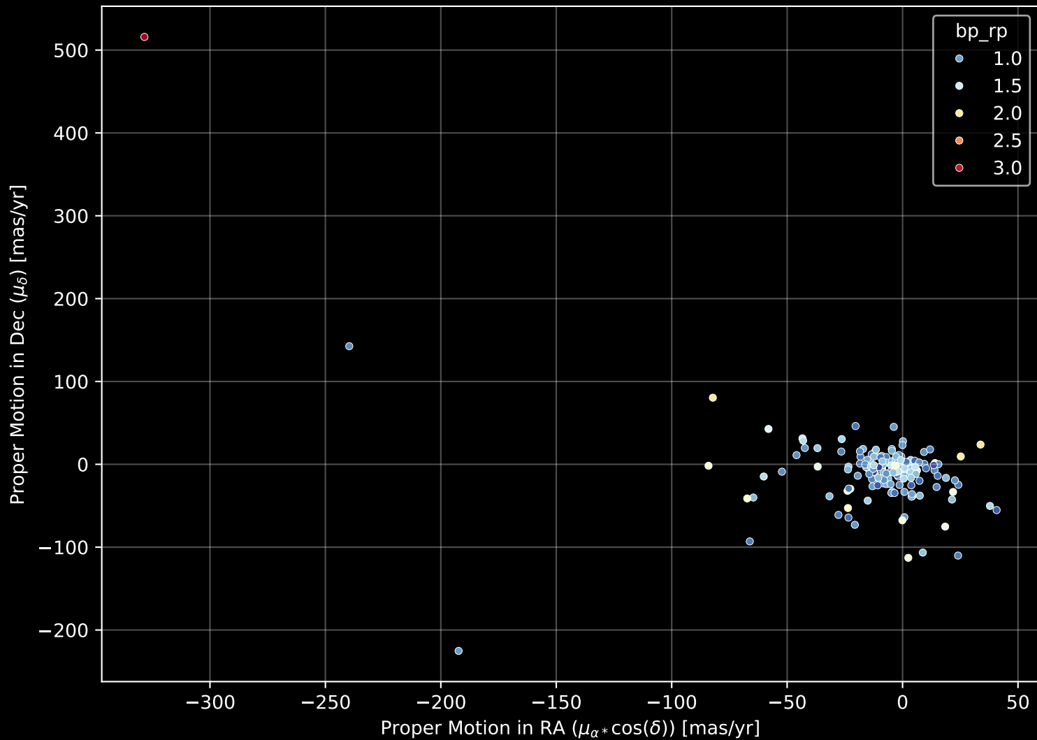
APOGEE DR17 Field: [038+48_MGA] Proper Motion Diagram (n= 159)
