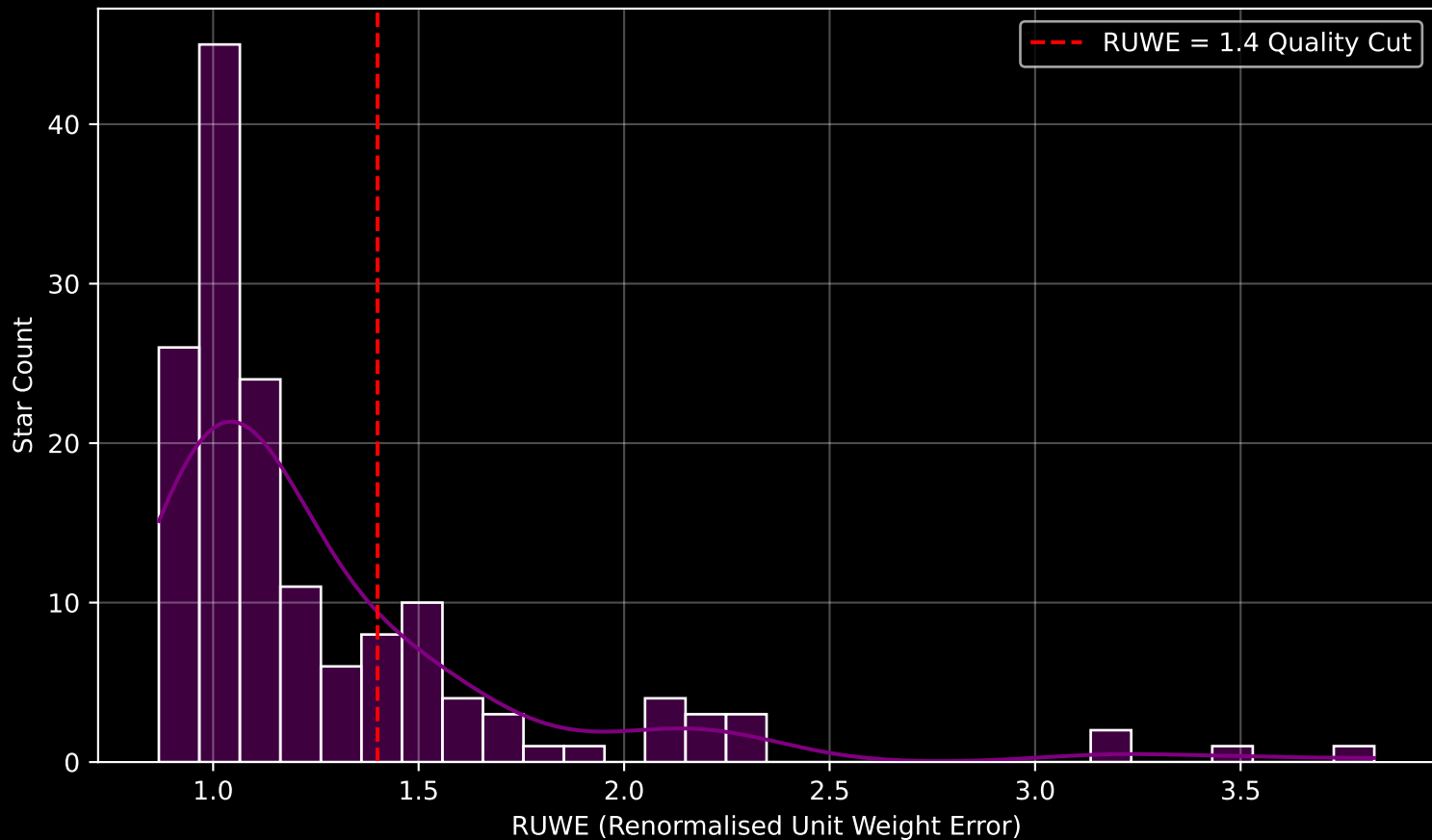
GAPOGEE DR17 Field [038+48_MGA] RUWE Distribution (n= 153)
