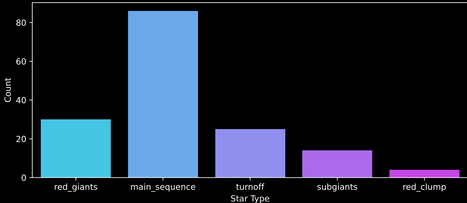
APOGEE DR17 Field: [038+48_MGA] Count plot of Star Type
